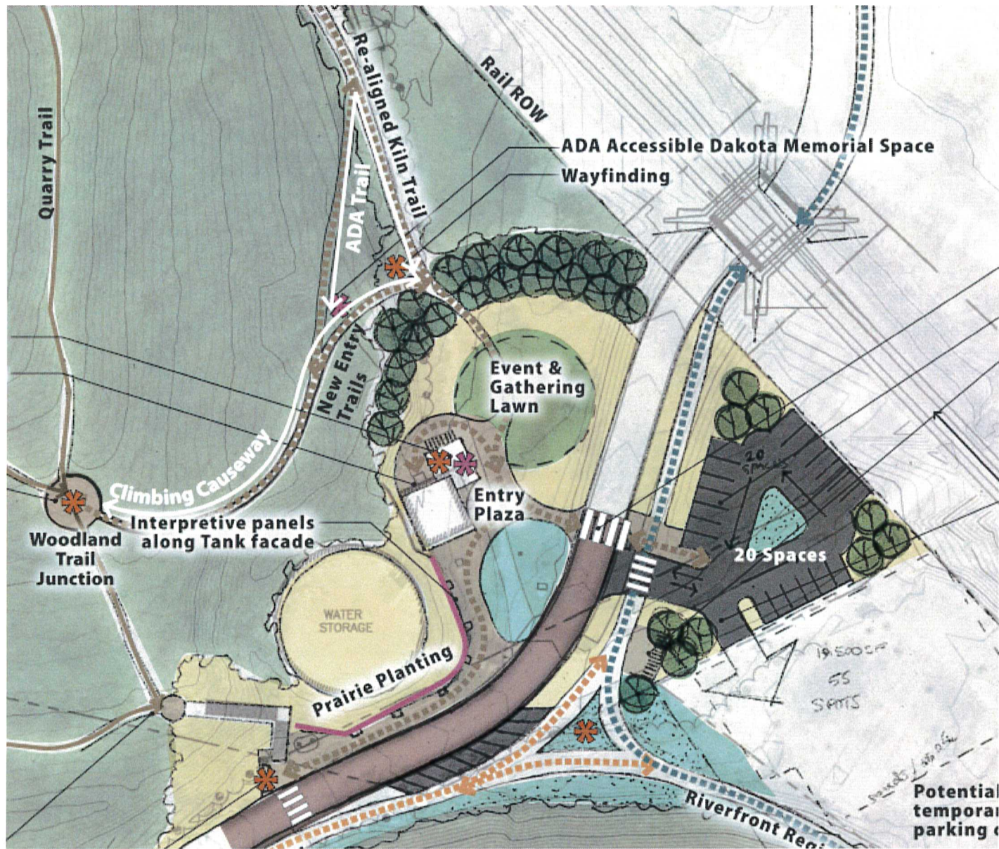
FIGURE 3.16 PARK ENTRY TRAILS
